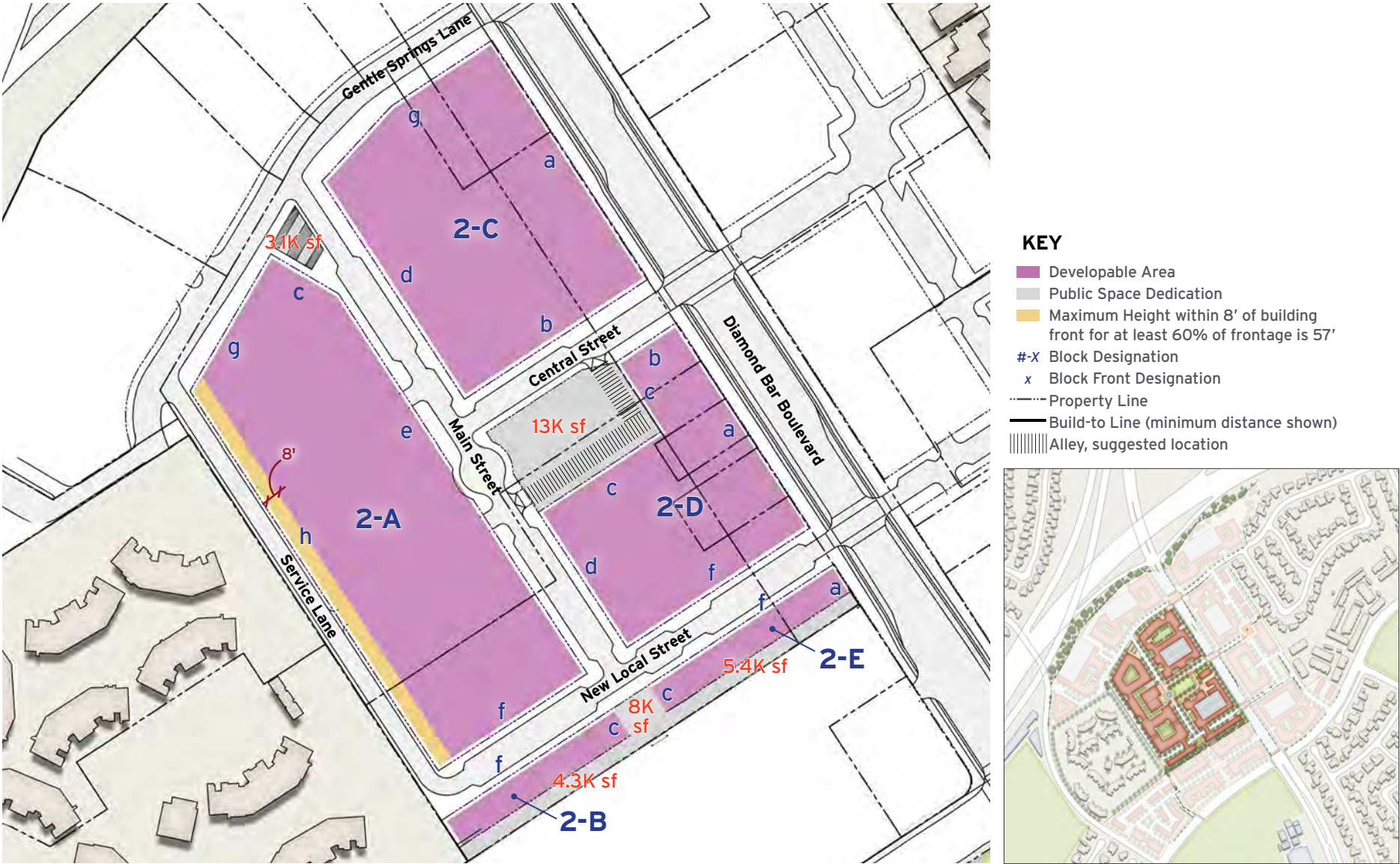
Figure 6-5 - Group 2 Block Development Diagram
