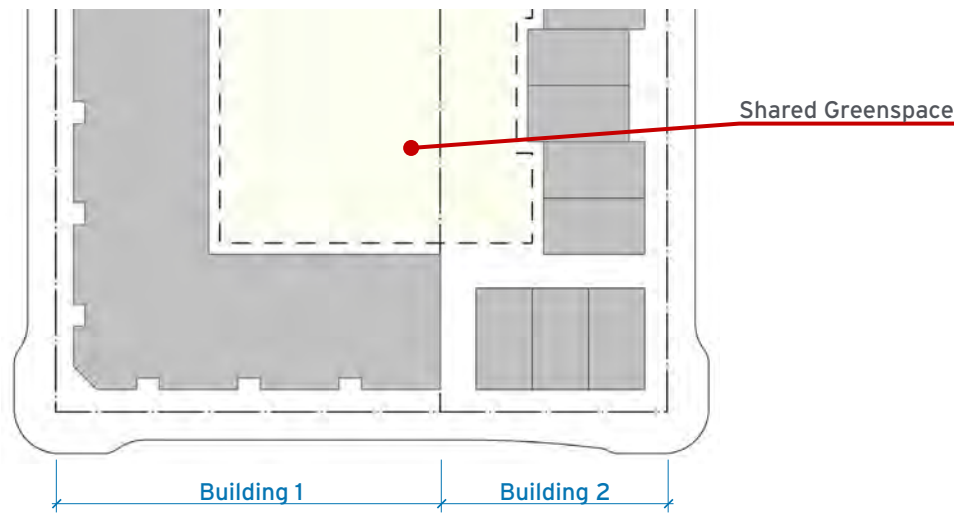
Figure 6-11 - Shared Outdoor Space Diagram Adjacent buildings may combine the required outdoor spaces into one shared space provided the cumulative minimum requirements for each building is met.
